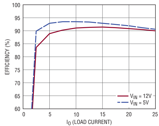
Figure 4. Measured Efficiency on Channel 2 ( V_{OUT2} = 1.5V , f_{SW} = 600kHz , Channel 1 Disabled)
